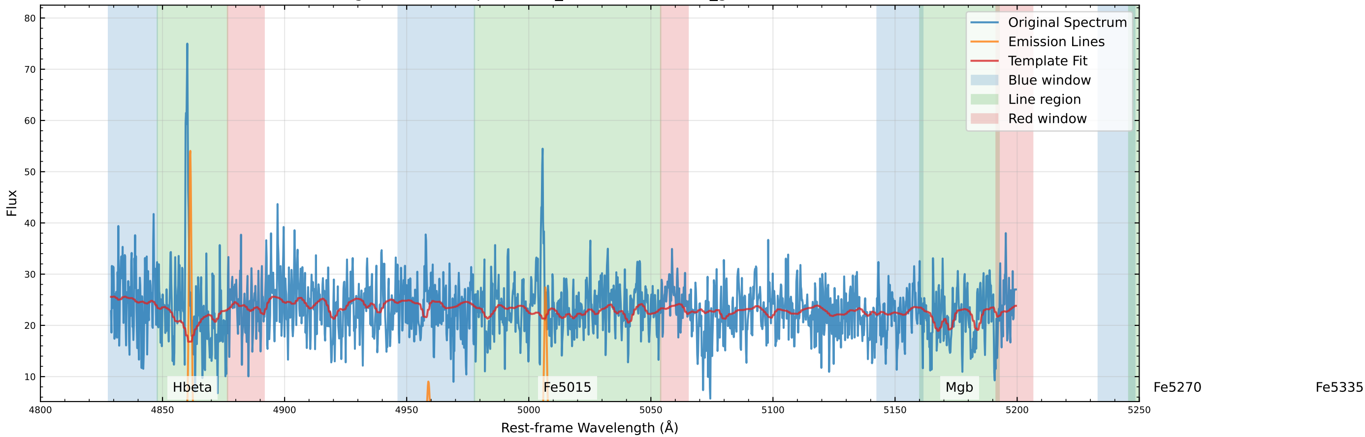
Original Data Comparison (v_star=-80.6 km/s, v_gas=-79.0 km/s)
