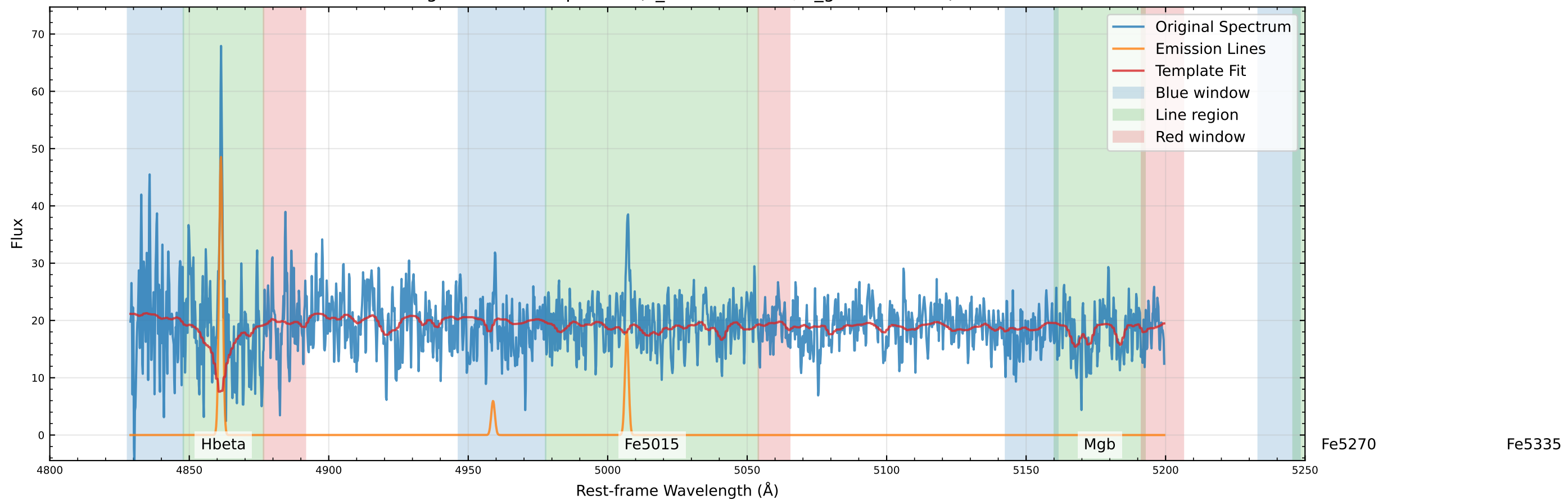
Original Data Comparison (v_star=9.4 km/s, v_gas=5.5 km/s)
