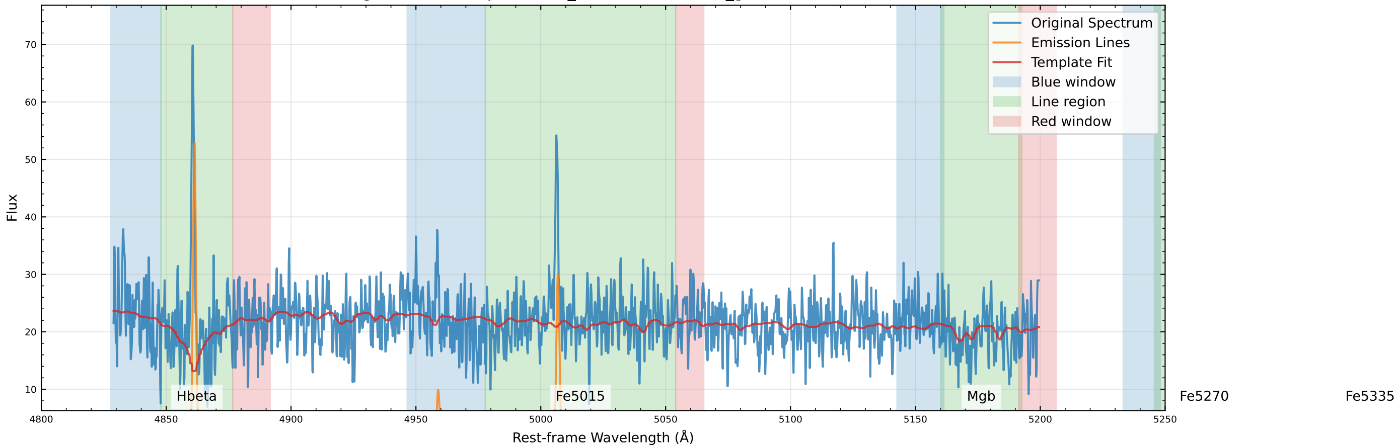
Original Data Comparison (v_star=-74.4 km/s, v_gas=-38.4 km/s)
