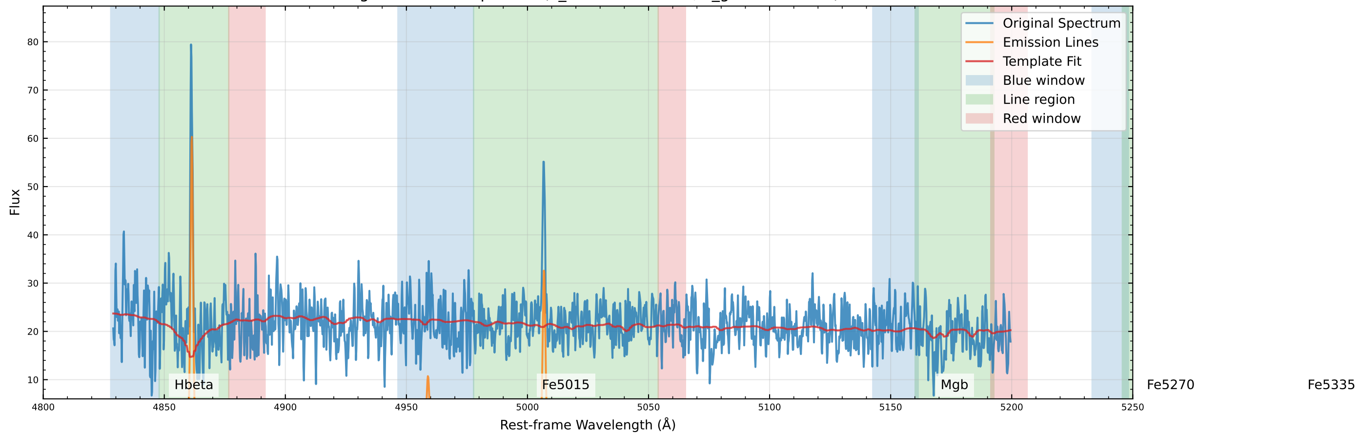
Original Data Comparison (v_star=-12.3 km/s, v_gas=-7.4 km/s)
