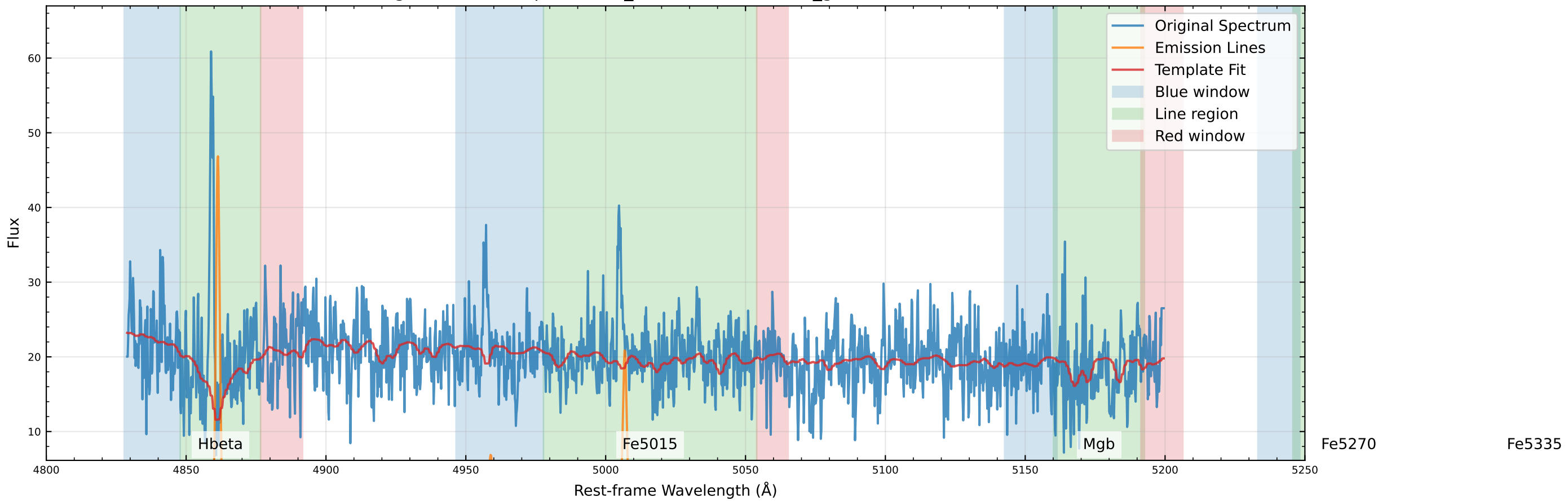
Original Data Comparison (v_star=-123.4 km/s, v_gas=-132.7 km/s)
