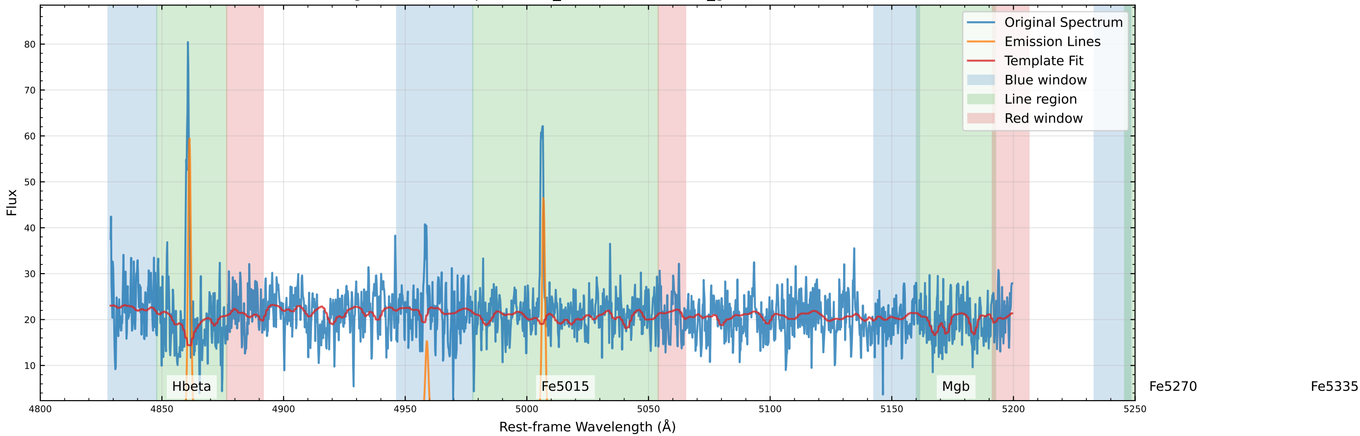
Original Data Comparison (v_star=-28.7 km/s, v_gas=-42.9 km/s)
