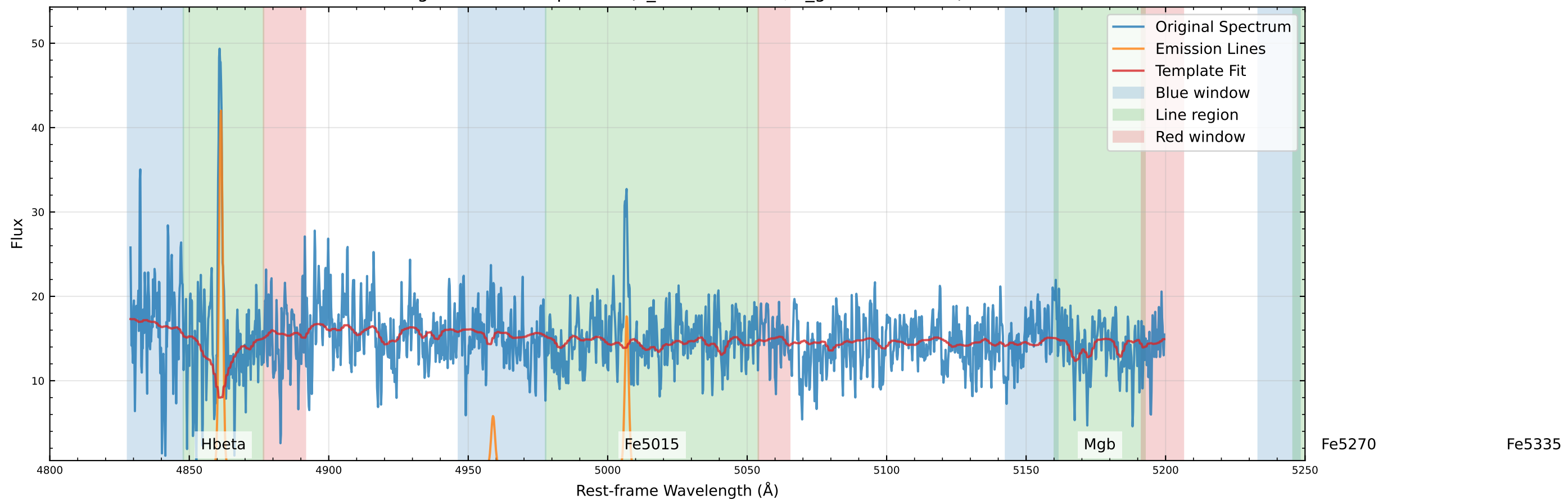
Original Data Comparison (v_star=8.5 km/s, v_gas=-14.8 km/s)
