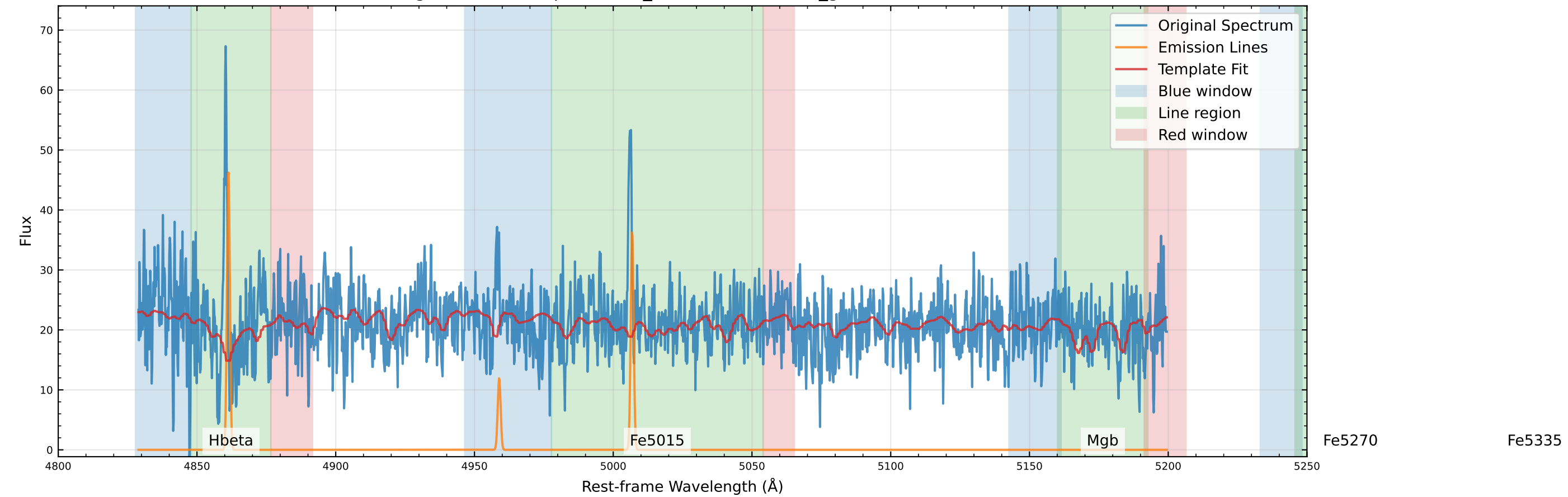
Original Data Comparison (v_star=-45.2 km/s, v_gas=-58.6 km/s)
