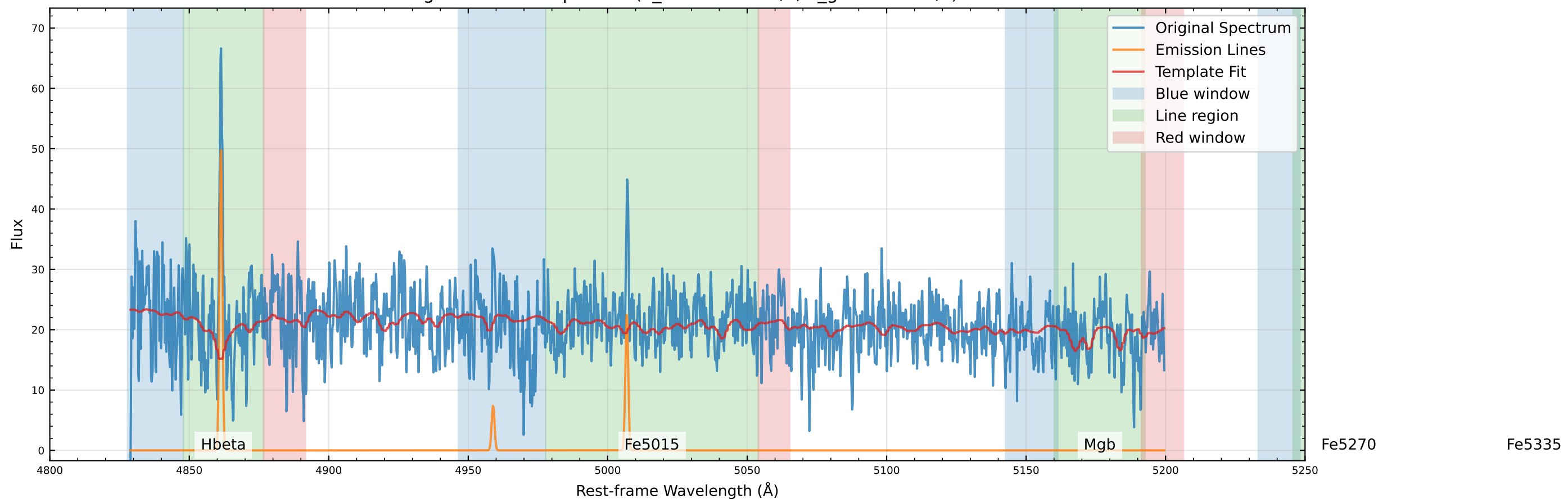
Original Data Comparison (v_star=-7.8 km/s, v_gas=5.7 km/s)
