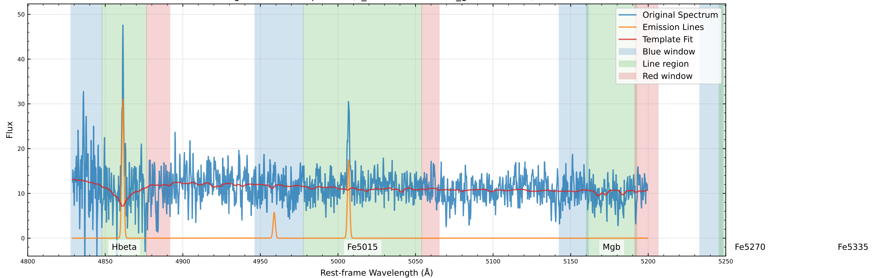
Original Data Comparison (v_star=12.0 km/s, v_gas=1.7 km/s)
