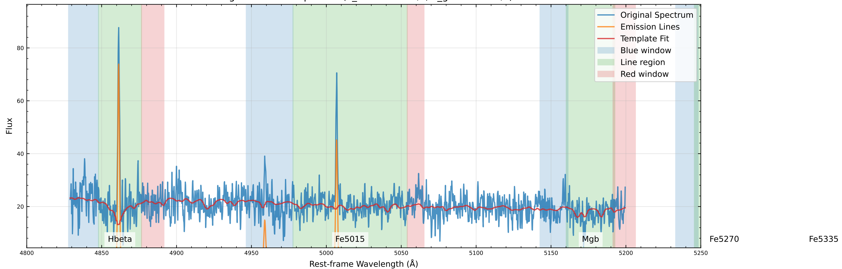
Original Data Comparison (v_star=0.9 km/s, v_gas=2.4 km/s)
