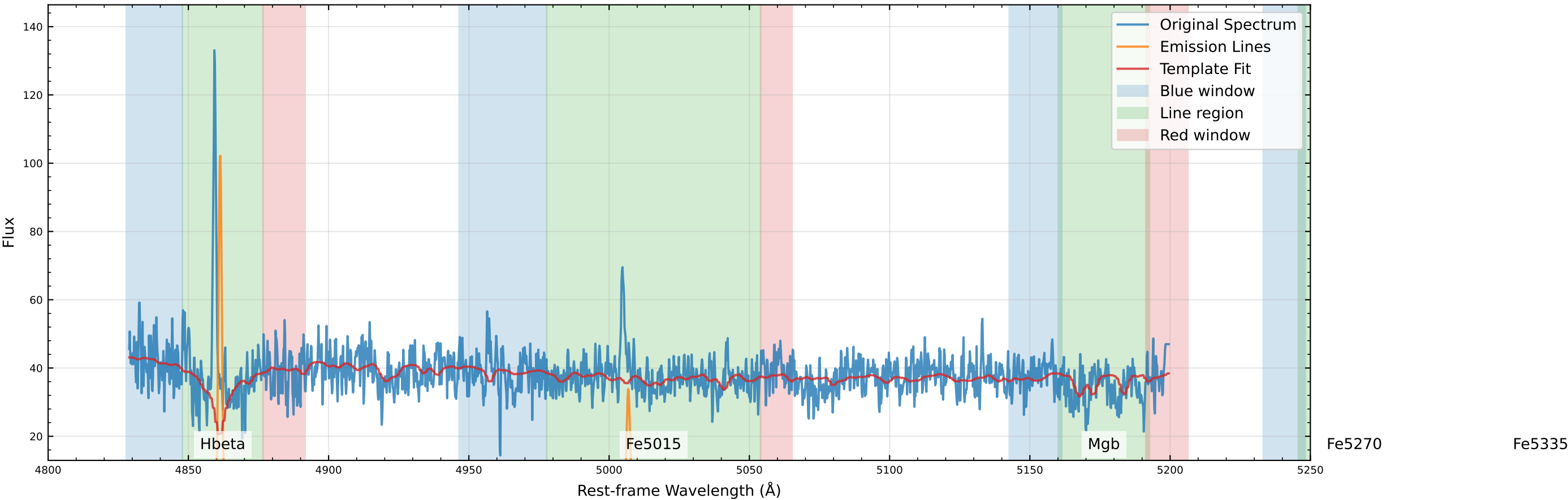
Original Data Comparison (v_star=-133.3 km/s, v_gas=-121.1 km/s)
