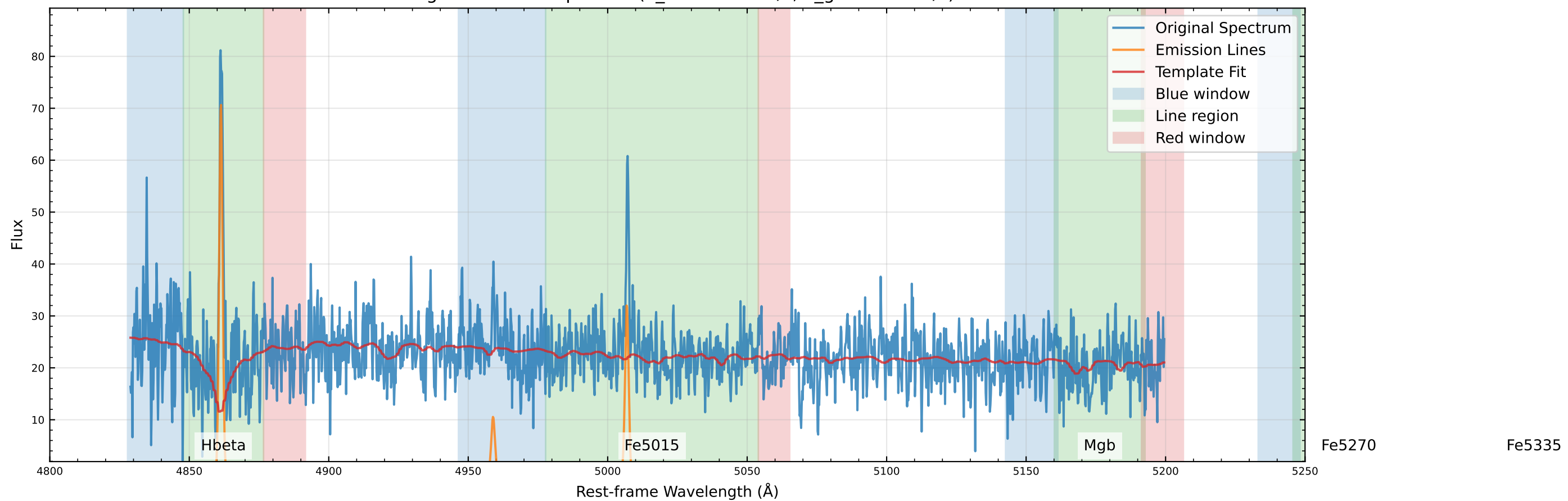
Original Data Comparison (v_star=0.7 km/s, v_gas=9.0 km/s)
