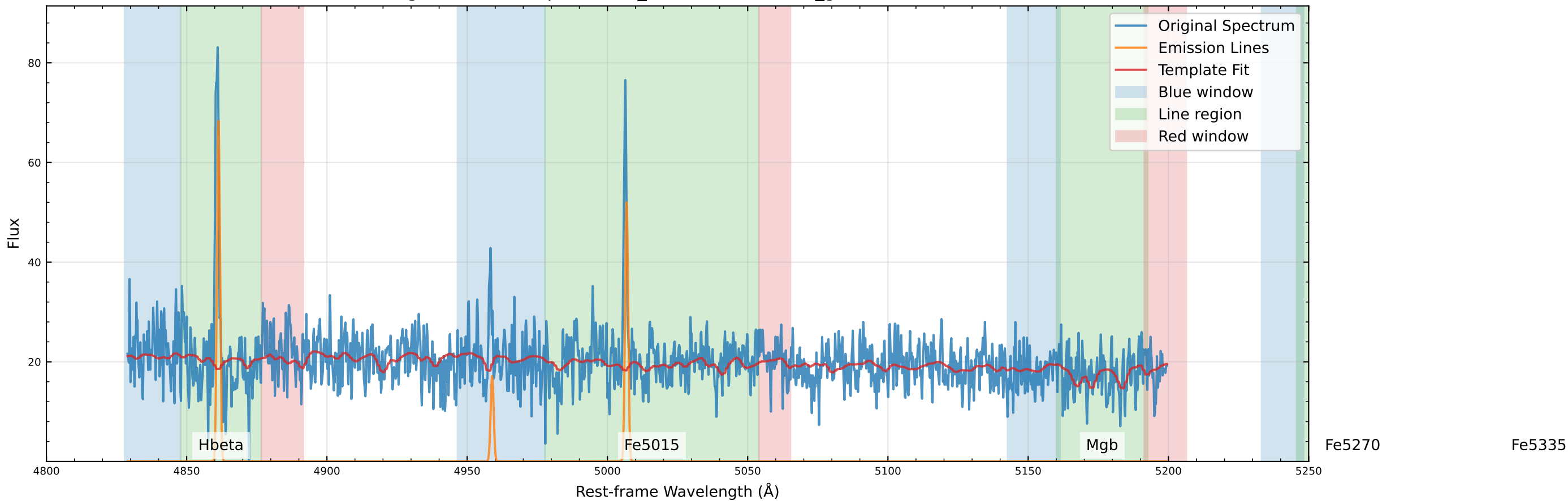
Original Data Comparison (v_star=-35.7 km/s, v_gas=-31.8 km/s)
