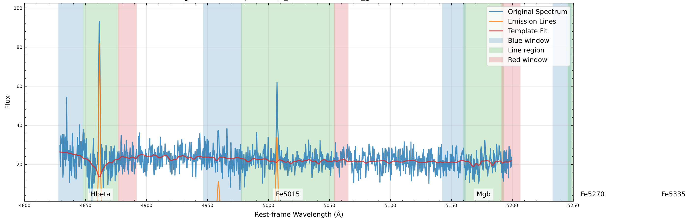
Original Data Comparison (v_star=-14.4 km/s, v_gas=-0.6 km/s)
