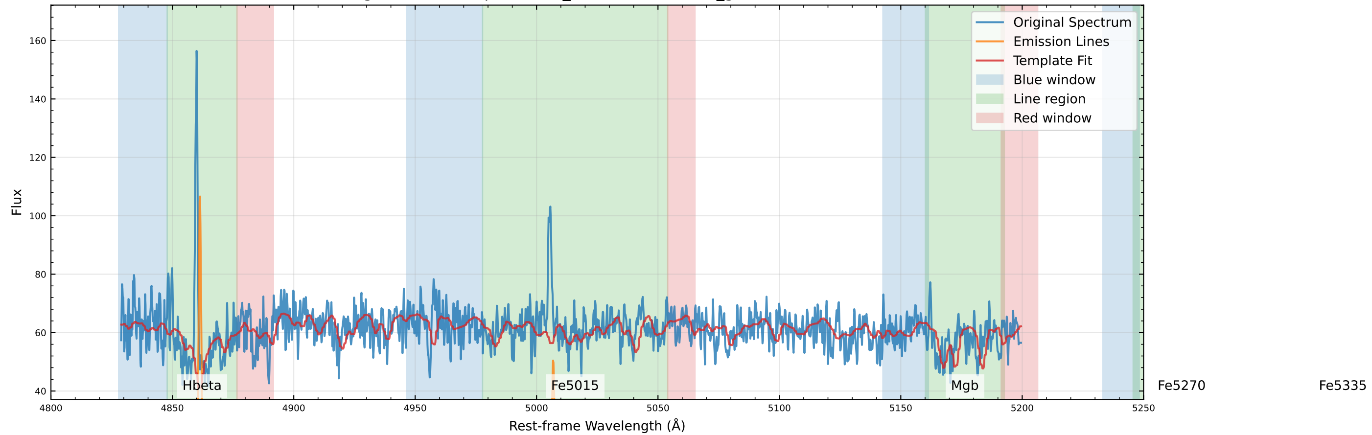
Original Data Comparison (v_star=-96.1 km/s, v_gas=-87.7 km/s)
