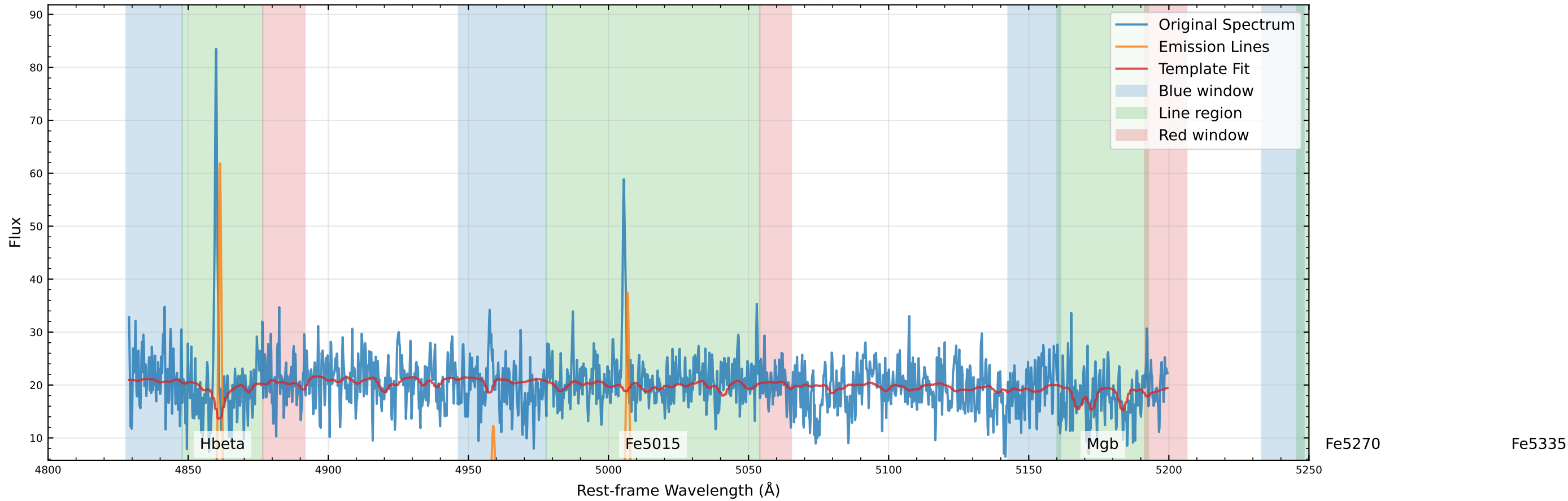
Original Data Comparison (v_star=-16.3 km/s, v_gas=-82.7 km/s)
