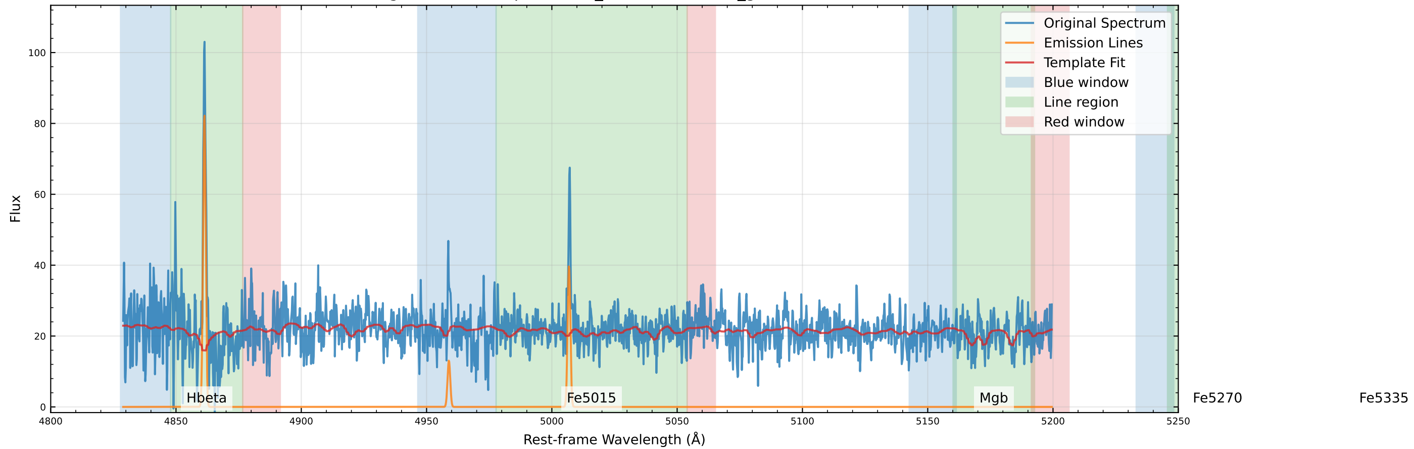
Original Data Comparison (v_star=1.4 km/s, v_gas=5.0 km/s)
