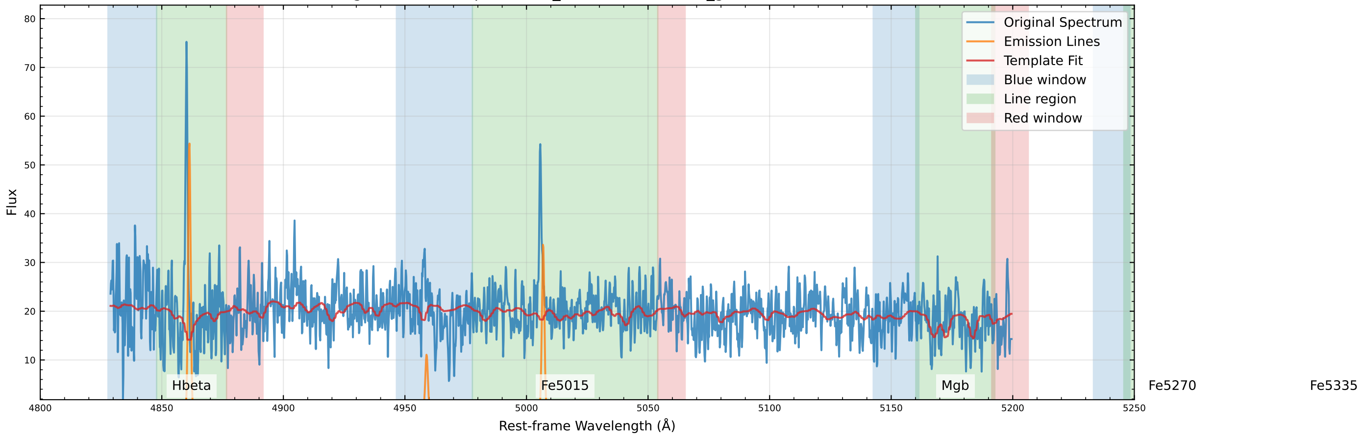
Original Data Comparison (v_star=-81.1 km/s, v_gas=-72.0 km/s)
