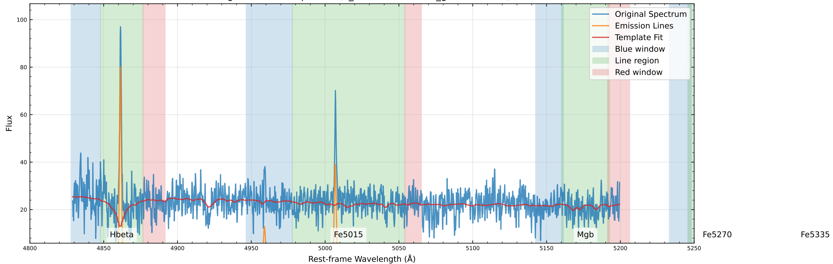
Original Data Comparison ( v_{\text{star}}=-3.9 km/s, v_{\text{gas}}=7.8 km/s)
