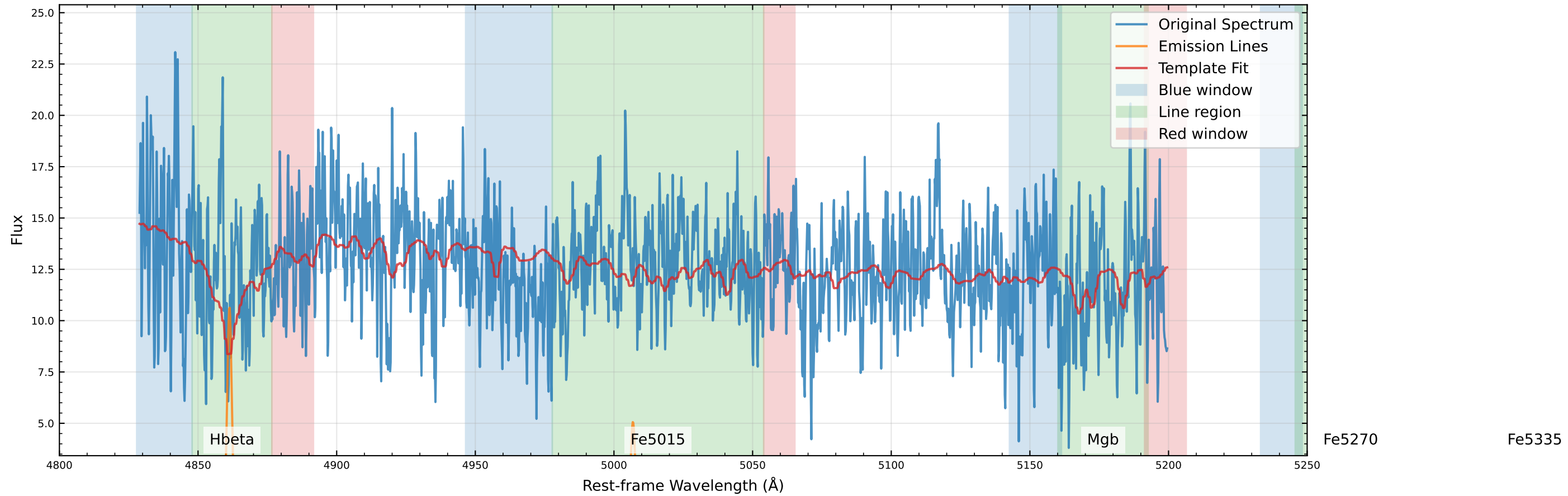
Original Data Comparison (v_star=-201.4 km/s, v_gas=-182.1 km/s)
