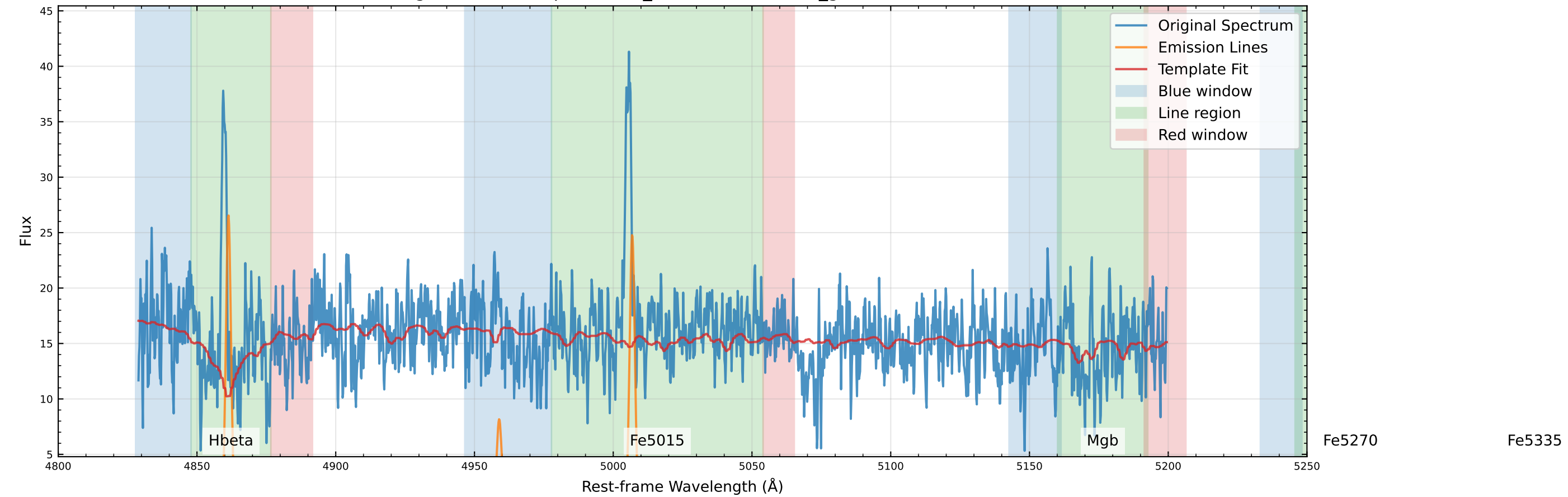
Original Data Comparison (v_star=-89.6 km/s, v_gas=-93.2 km/s)
