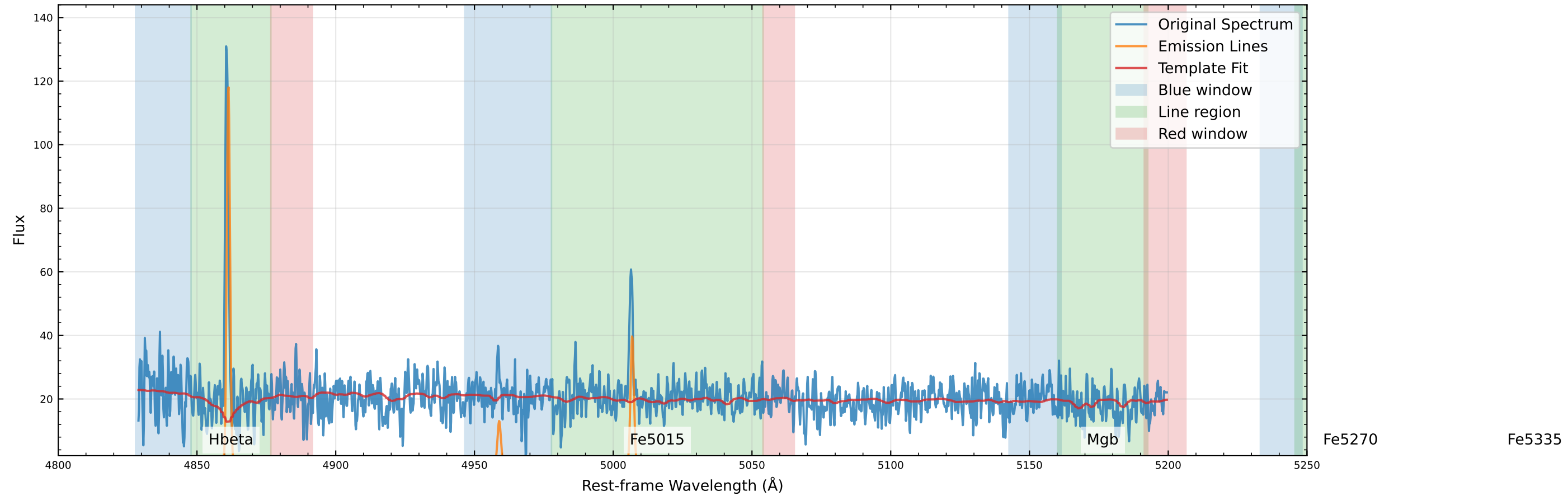
Original Data Comparison (v_star=-99.3 km/s, v_gas=-36.3 km/s)
