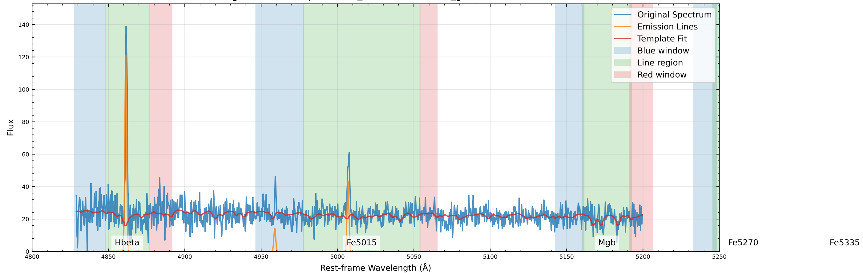
Original Data Comparison (v_star=26.4 km/s, v_gas=25.6 km/s)
