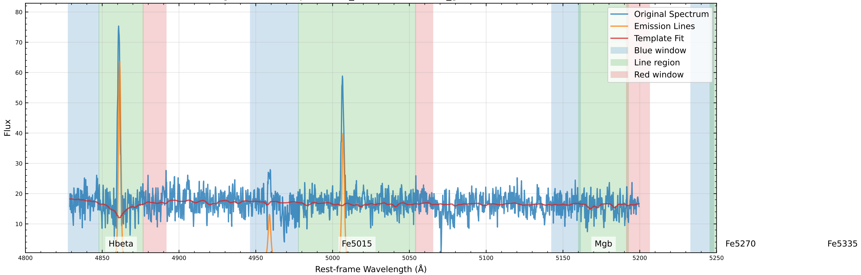
Original Data Comparison (v_star=-71.7 km/s, v_gas=-29.3 km/s)
