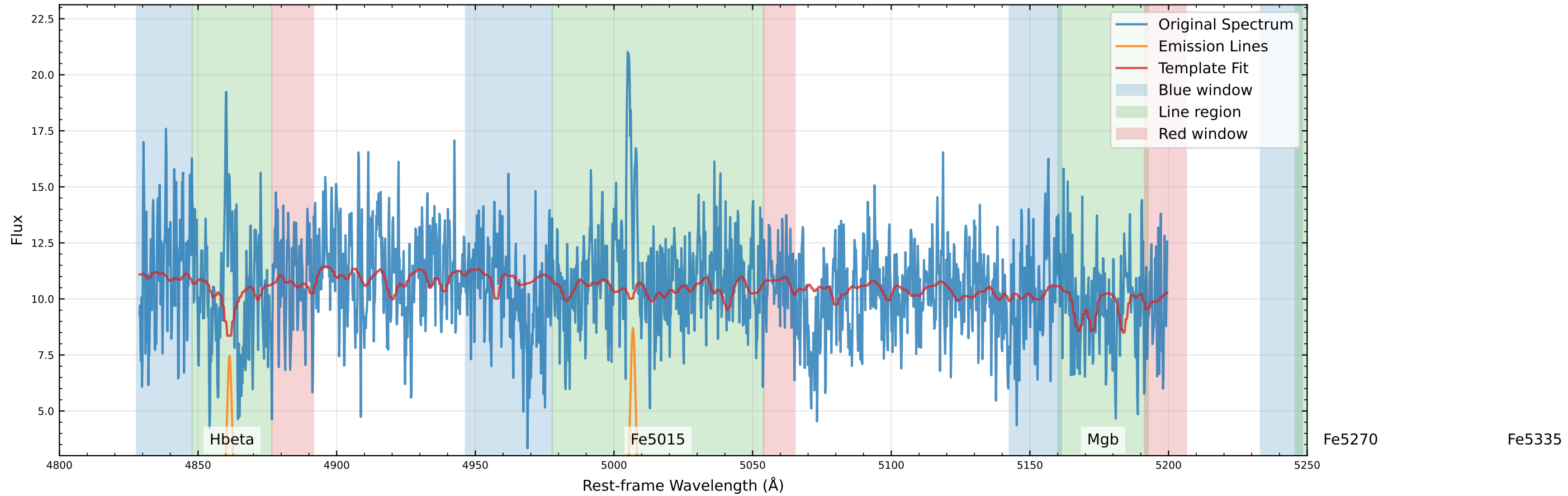
Original Data Comparison (v_star=-69.4 km/s, v_gas=-72.3 km/s)
