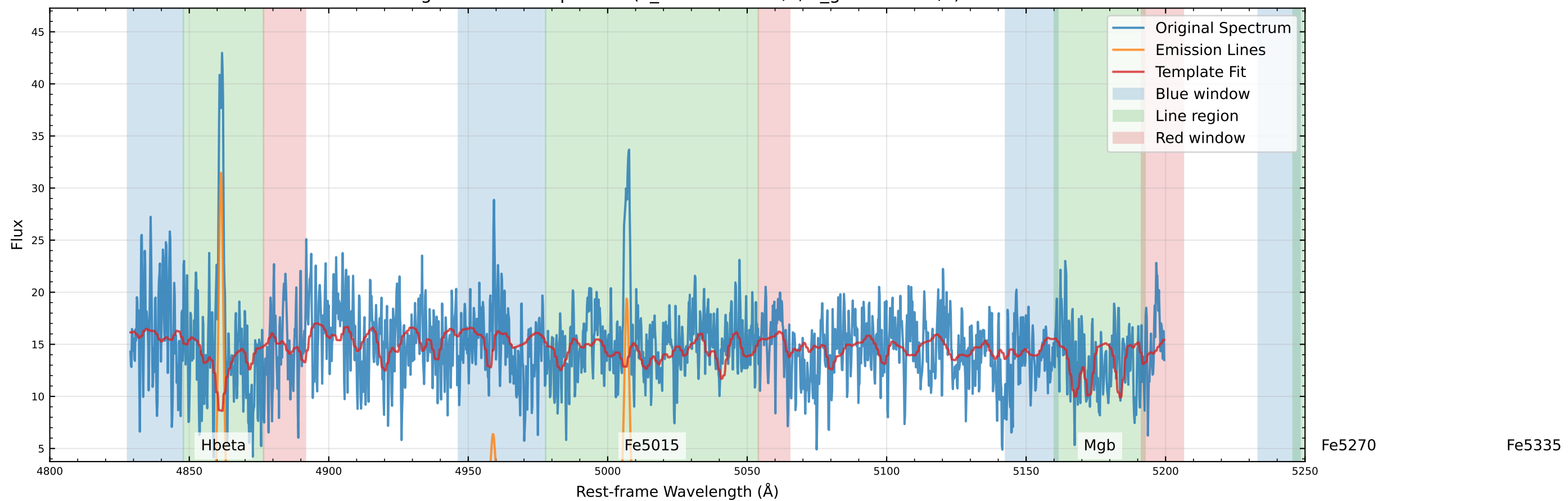
Original Data Comparison (v_star=76.5 km/s, v_gas=6.0 km/s)
