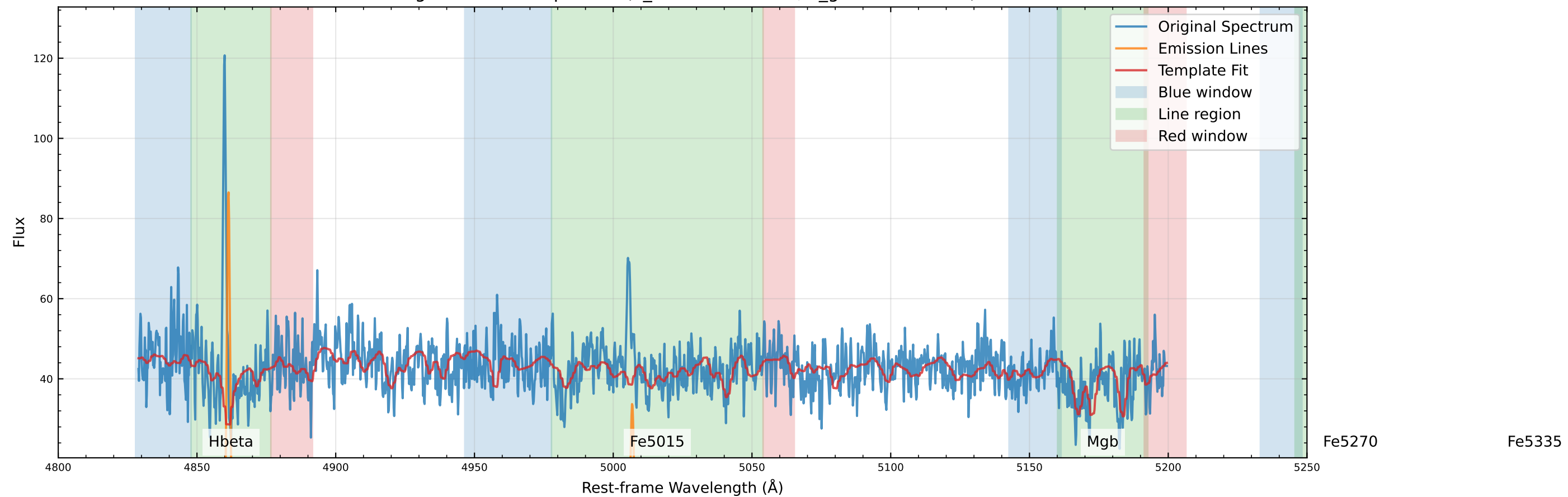
Original Data Comparison (v_star=-80.3 km/s, v_gas=-85.7 km/s)
