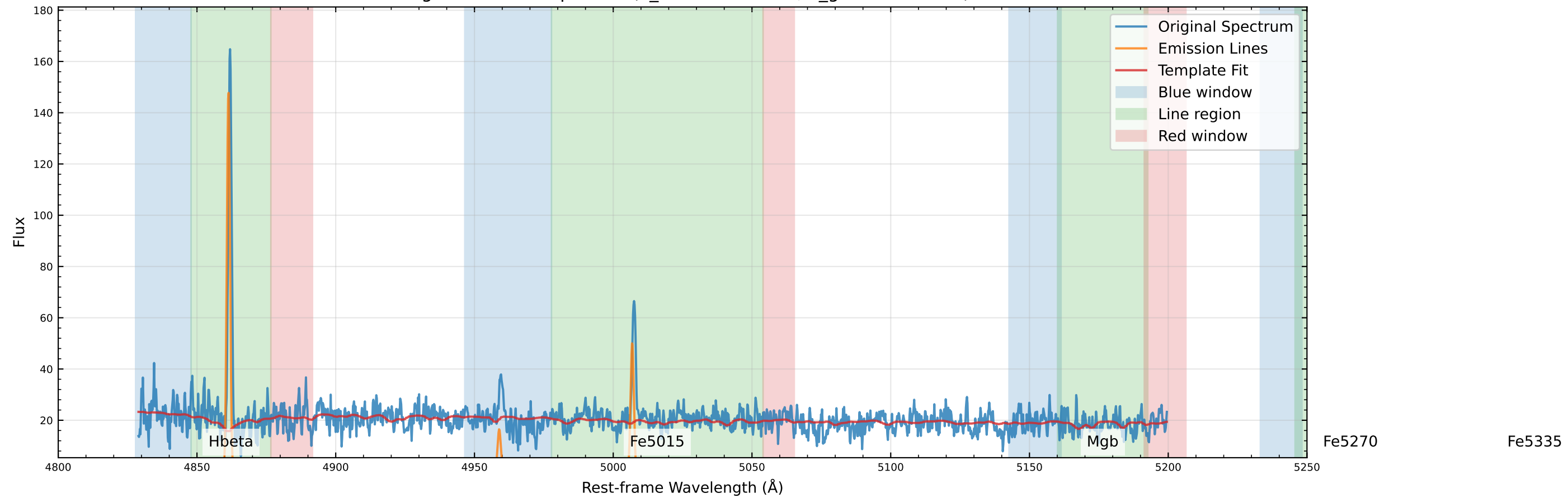
Original Data Comparison (v_star=48.3 km/s, v_gas=34.9 km/s)
