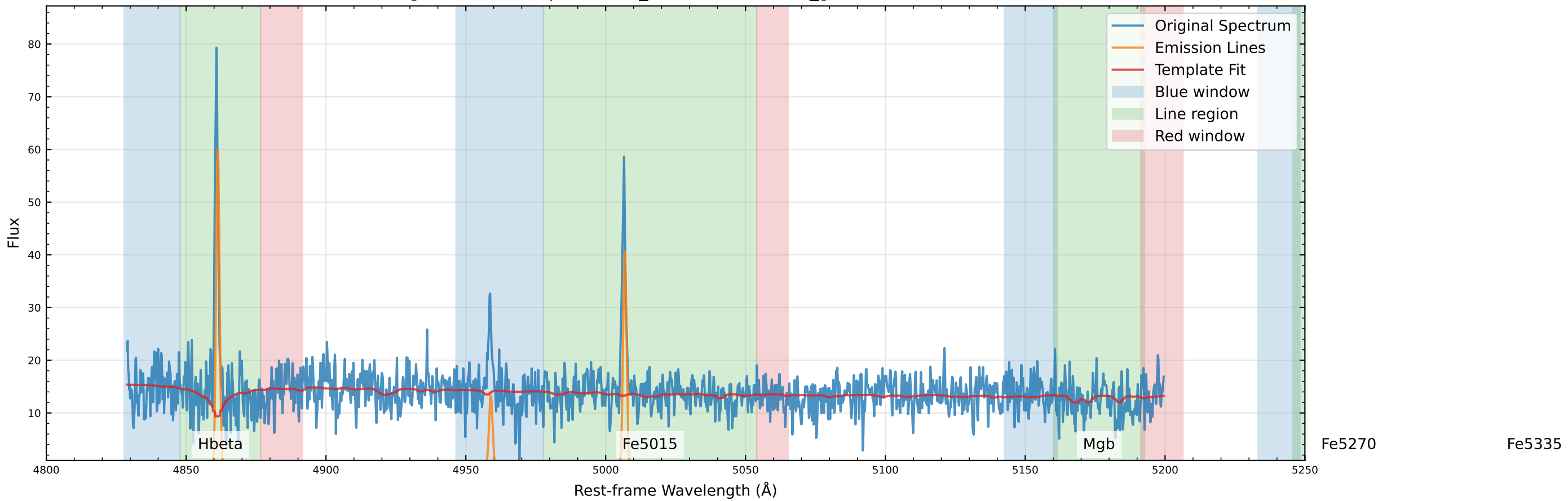
Original Data Comparison (v_star=60.0 km/s, v_gas=-27.4 km/s)
