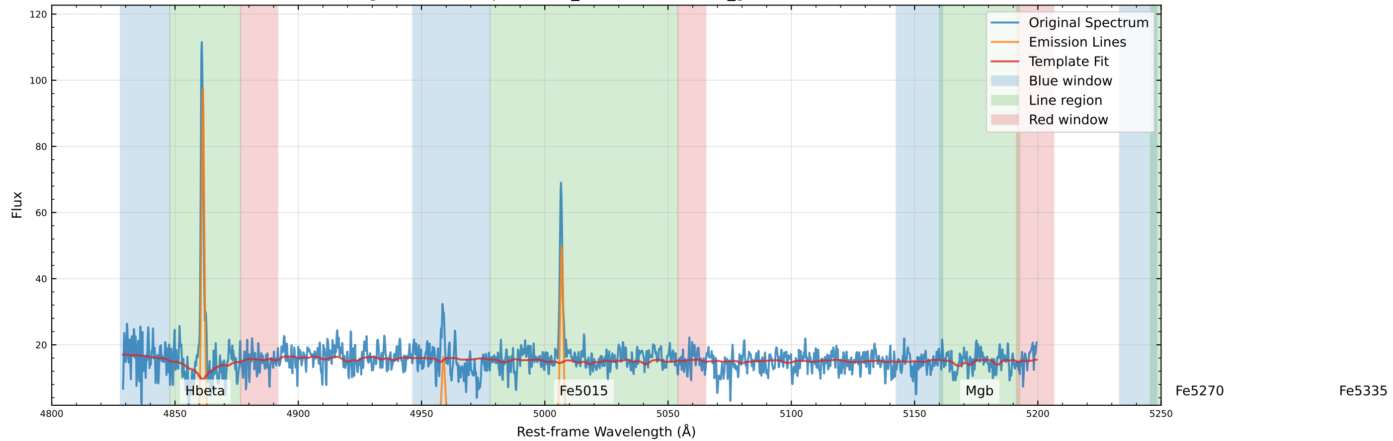
Original Data Comparison (v_star=-55.3 km/s, v_gas=-20.2 km/s)
