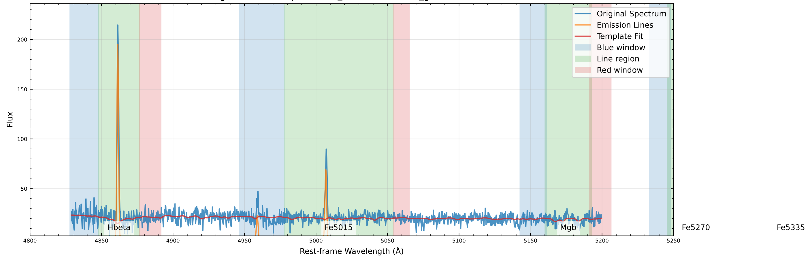
Original Data Comparison (v_star=4.0 km/s, v_gas=12.5 km/s)
