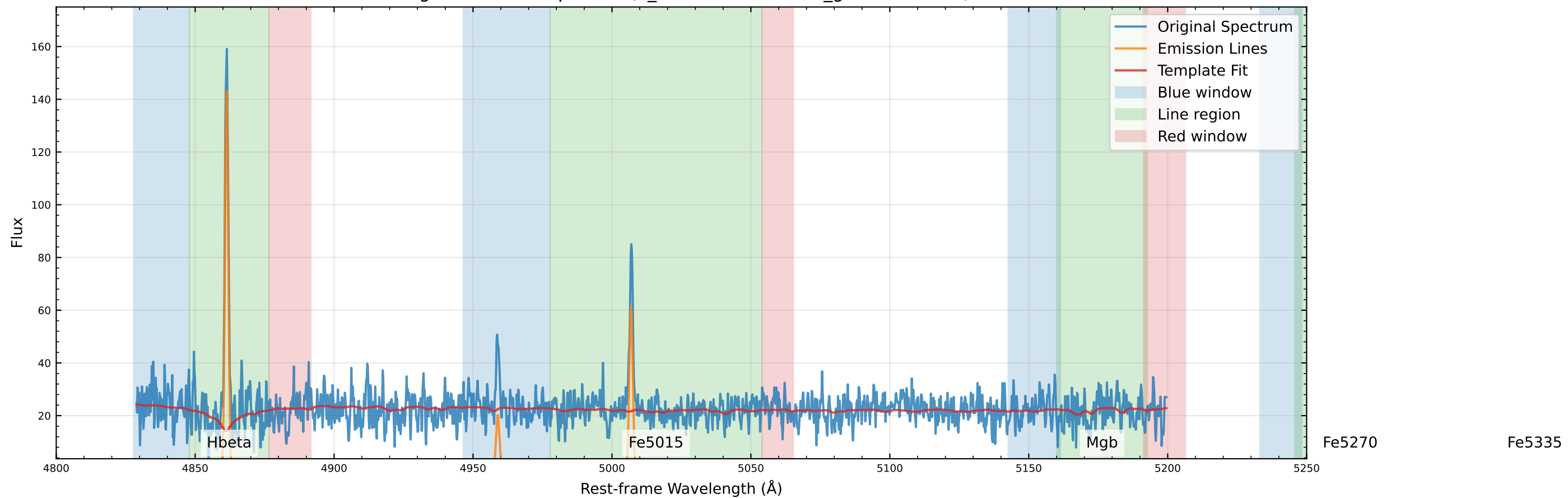
Original Data Comparison (v_star=-35.3 km/s, v_gas=-0.3 km/s)
