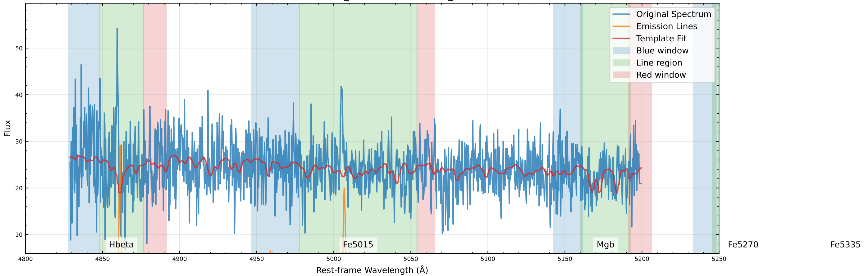
Original Data Comparison (v_star=-135.1 km/s, v_gas=-107.4 km/s)
