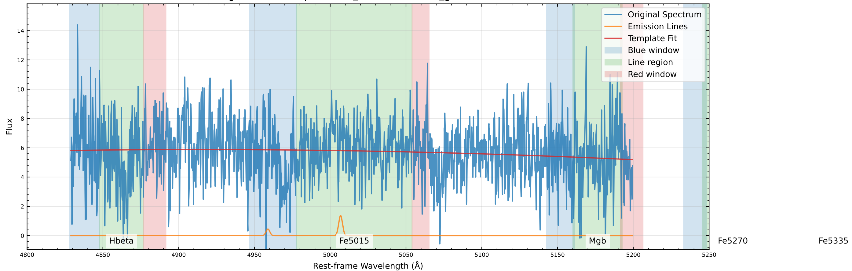
Original Data Comparison (v_star=0.0 km/s, v_gas=93.4 km/s)
