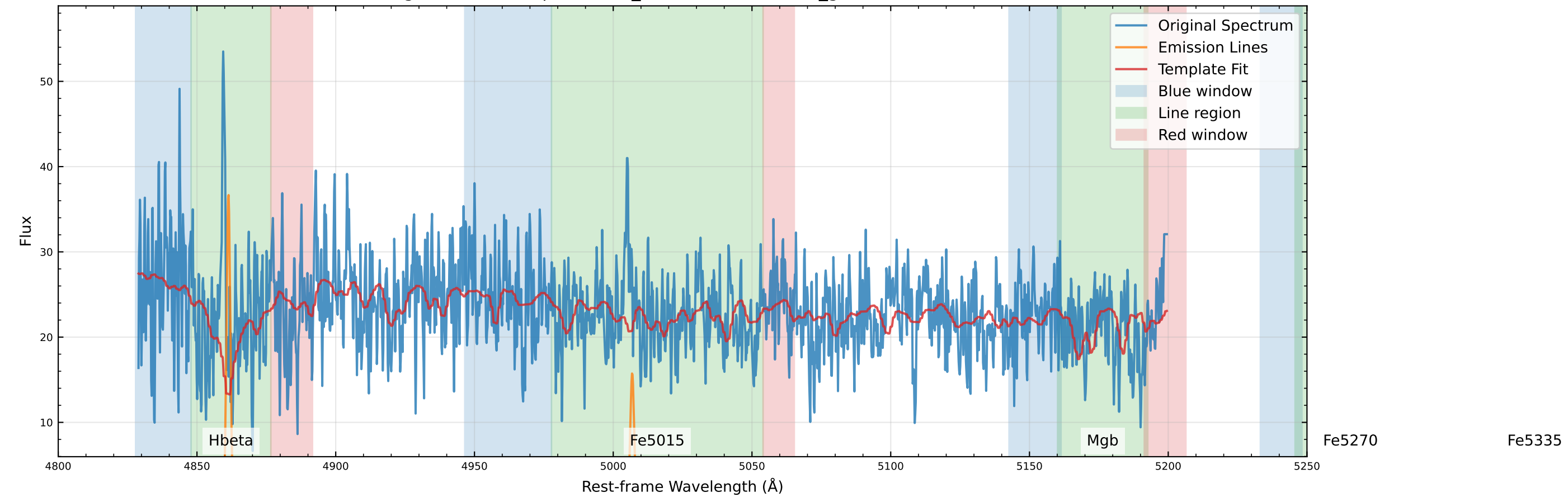
Original Data Comparison (v_star=-112.4 km/s, v_gas=-113.4 km/s)
