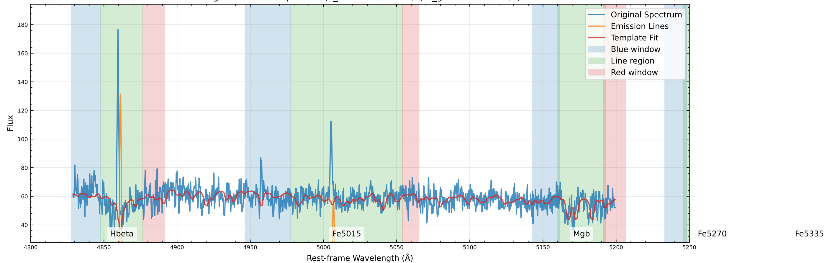
Original Data Comparison (v_star=-105.3 km/s, v_gas=-104.0 km/s)
