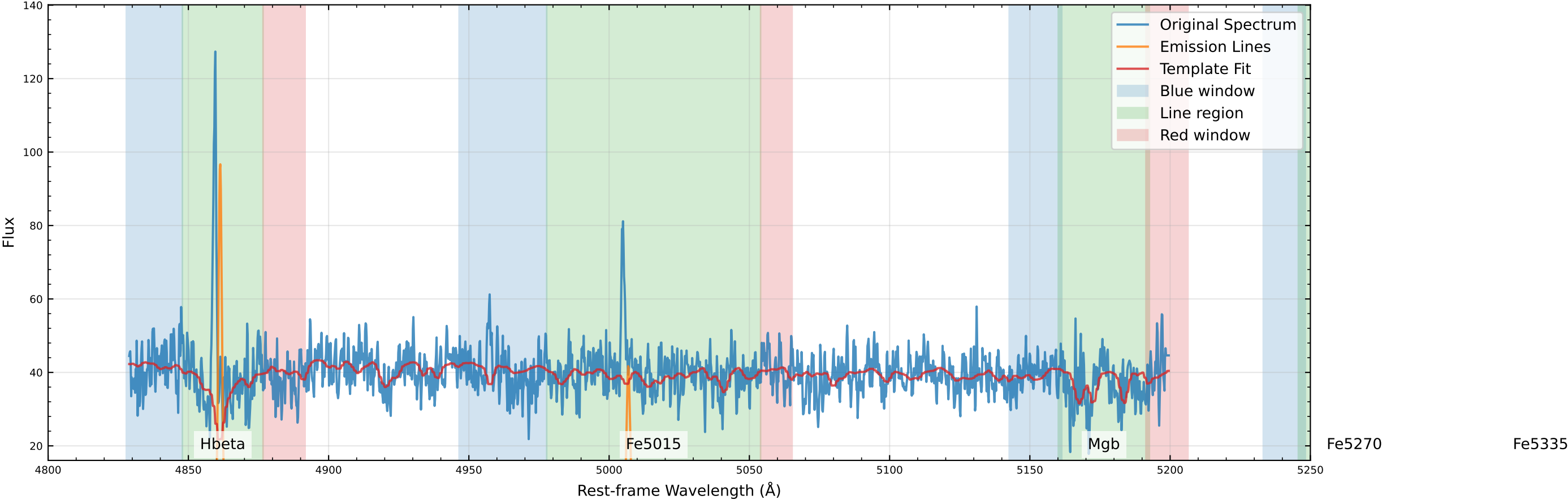
Original Data Comparison (v_star=-110.0 km/s, v_gas=-119.5 km/s)
