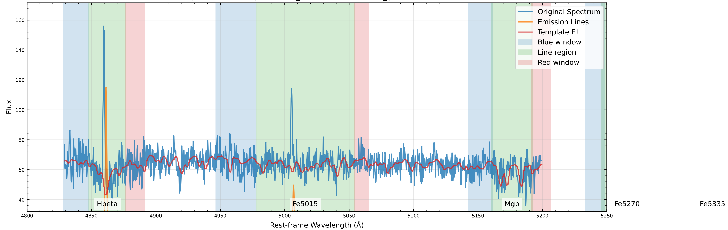
Original Data Comparison (v_star=-108.8 km/s, v_gas=-99.6 km/s)
