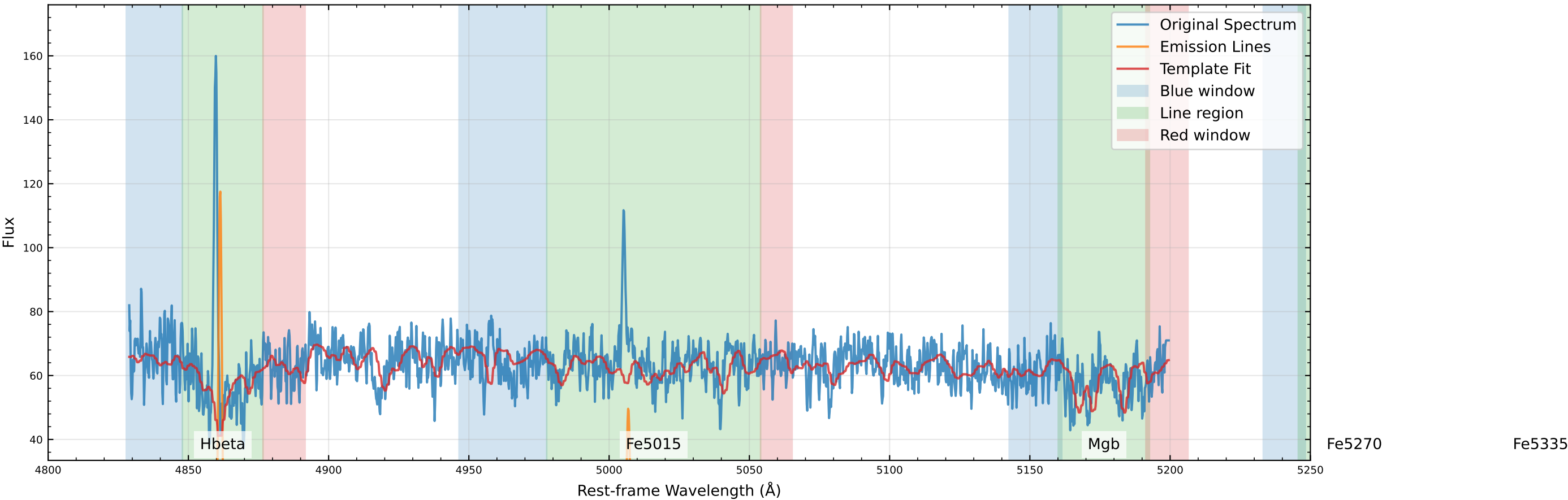
Original Data Comparison (v_star=-113.4 km/s, v_gas=-100.0 km/s)
