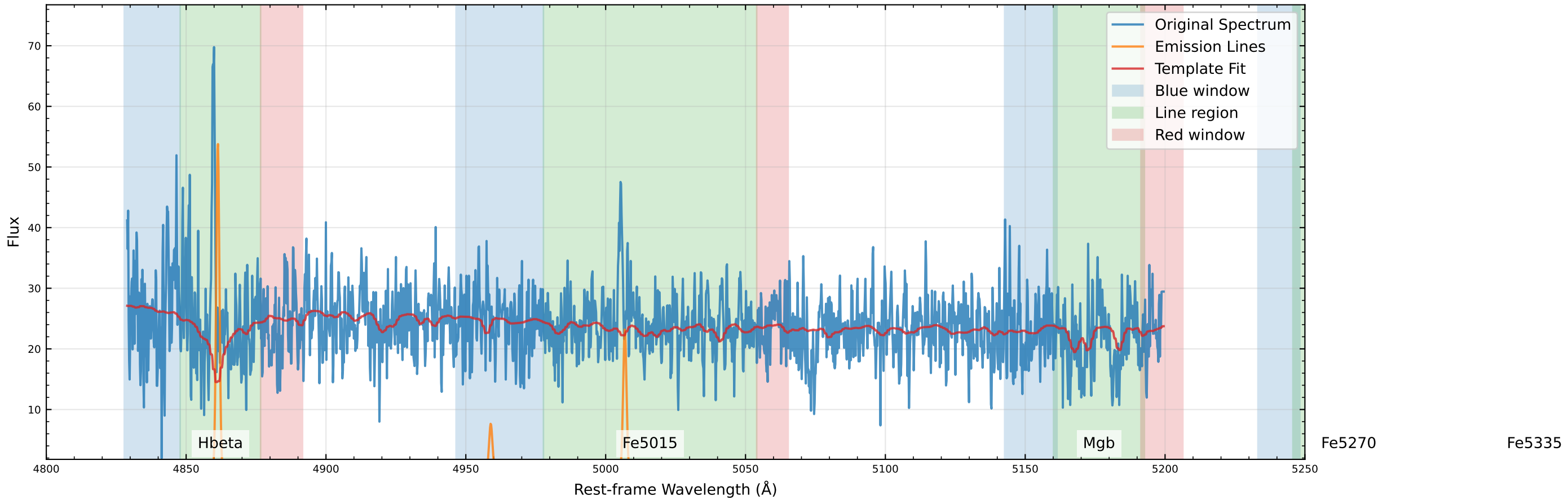
Original Data Comparison (v_star=-87.8 km/s, v_gas=-96.5 km/s)
