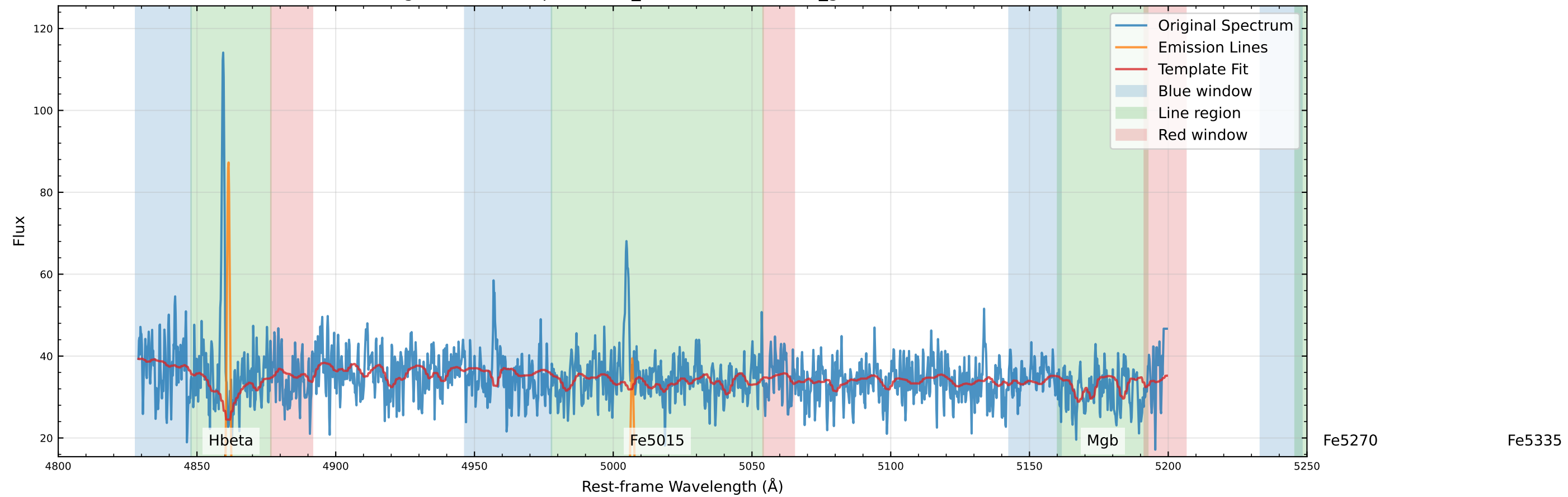
Original Data Comparison (v_star=-113.3 km/s, v_gas=-120.4 km/s)
