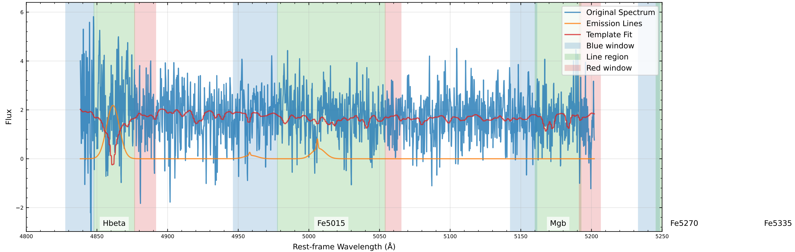
Original Data Comparison (v_star=538.5 km/s, v_gas=544.6 km/s)
