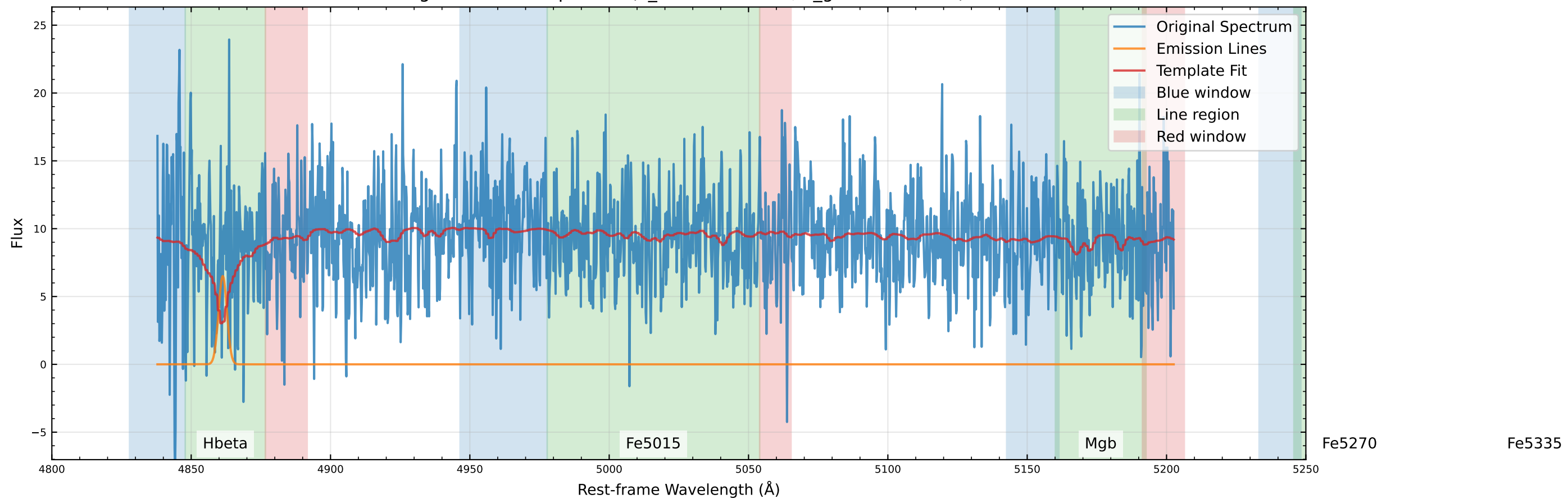
Original Data Comparison (v_star=-7.8 km/s, v_gas=71.6 km/s)
