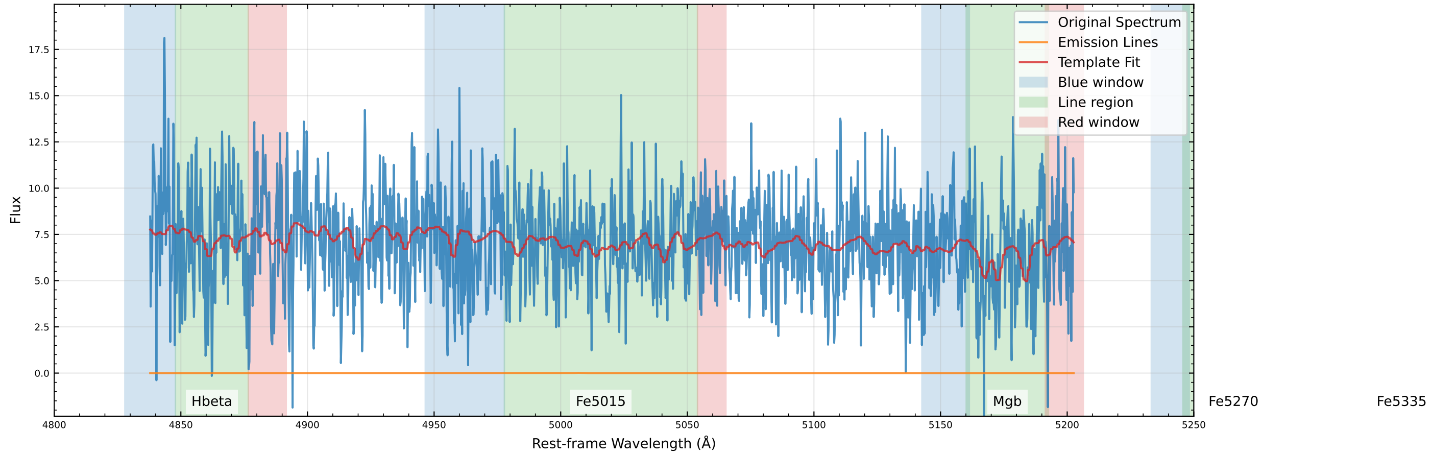
Original Data Comparison (v_star=-13.3 km/s, v_gas=-13.3 km/s)
