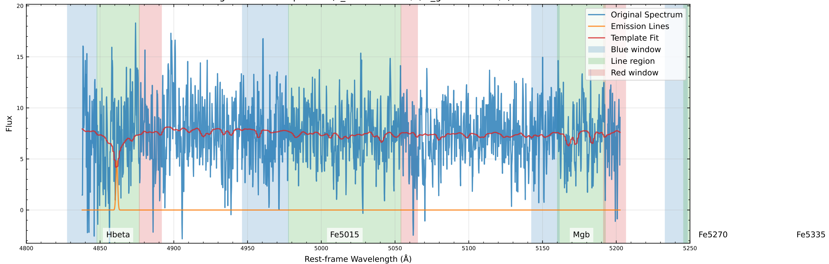
Original Data Comparison (v_star=36.5 km/s, v_gas=41.6 km/s)
