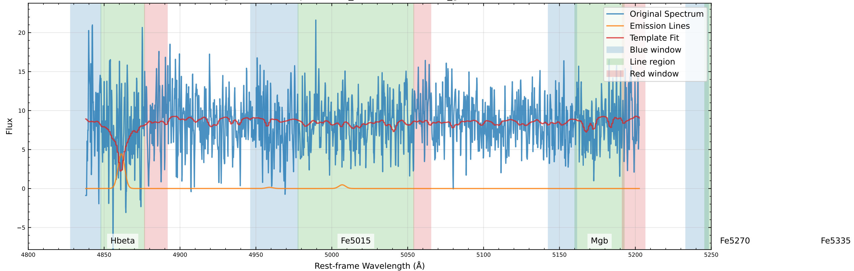
Original Data Comparison (v_star=152.1 km/s, v_gas=93.1 km/s)
