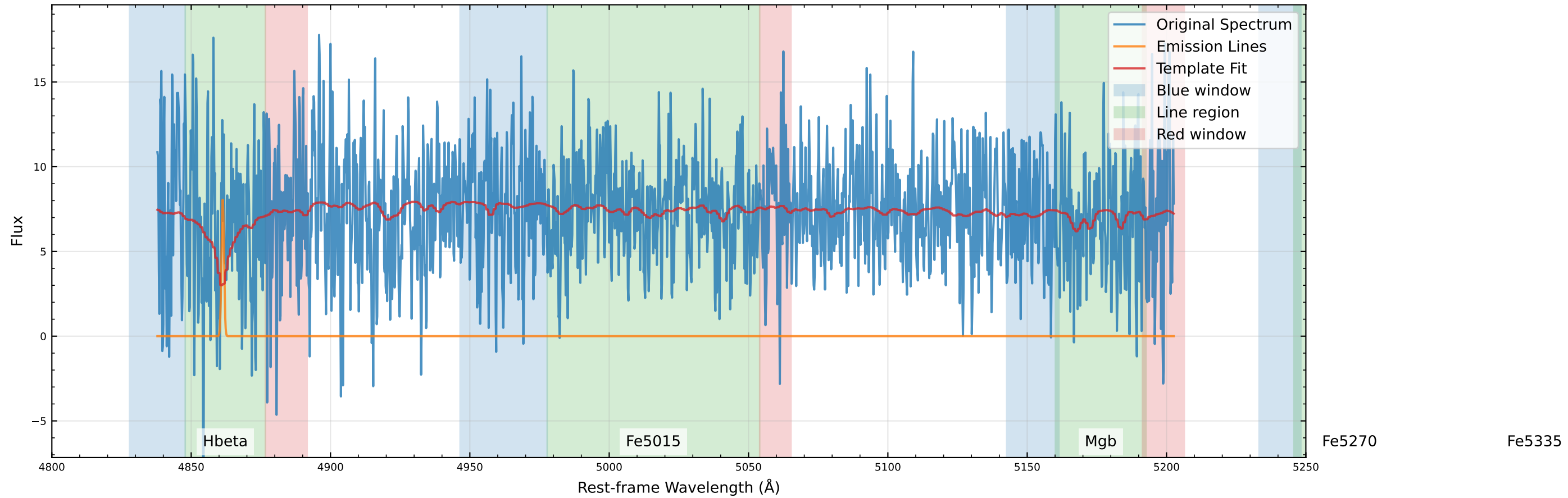
Original Data Comparison (v_star=17.4 km/s, v_gas=4.4 km/s)
