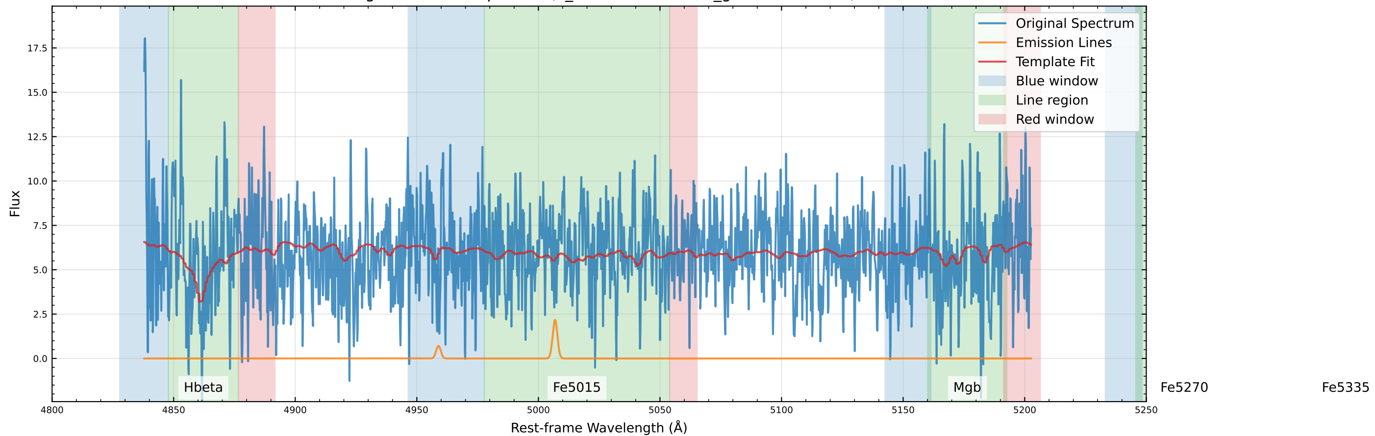
Original Data Comparison (v_star=60.3 km/s, v_gas=155.0 km/s)
