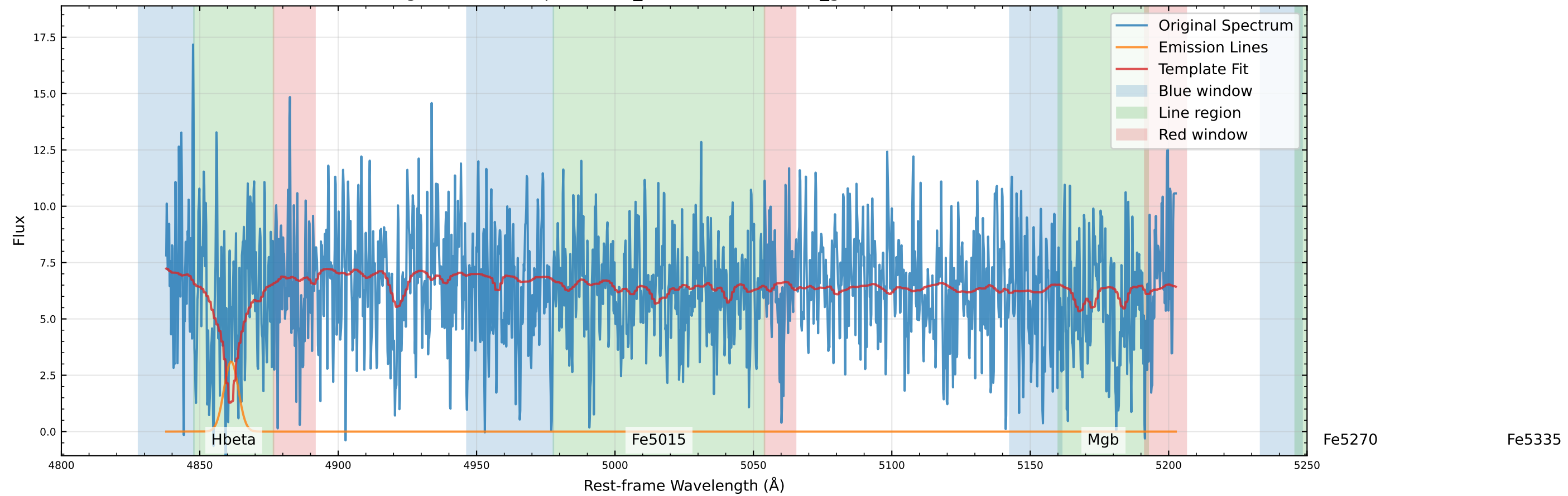
Original Data Comparison (v_star=-105.8 km/s, v_gas=-115.0 km/s)
